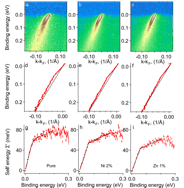
FIG. 2 (color online). (a)–(c) Photoemission intensity distributions along the BZ diagonal. (a) Pure BSCCO, (b) Ni substituted, and (c) Zn substituted BSCCO. The middle row shows corresponding experimental dispersion. In the last row, the real part of the self-energy obtained by subtractions of the bare band is displayed. The black solid lines are guides to eye, while the red symbols represent the data points.
